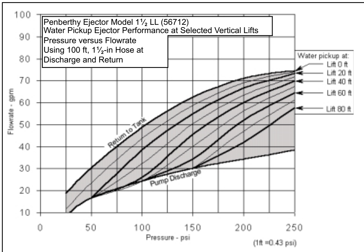
Figure A3—Penberthy Model 1½ LL (56712) water pickup ejector performance graph.
