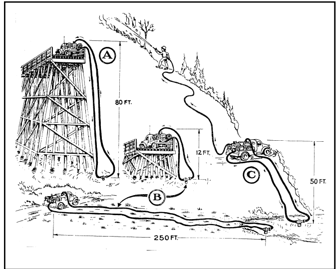
Figure 11—Ejectors are designed for different uses: (a) high lift, (b) low lift, and (c) moderate lift with long lines.
