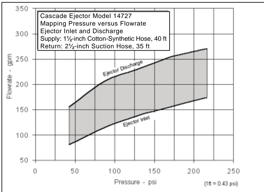
Figure A9—Cascade Ejector Model 14727 mapping pressure versus flow rate graph.
