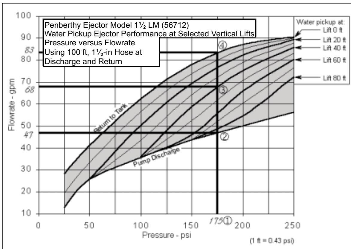
Figure A—Ejector exercise example for discussion.
