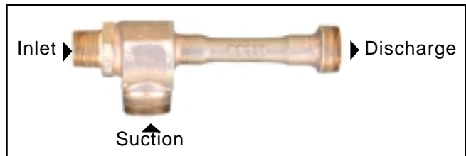
Figure E6—Penberthy Ejector Model 1¼ LH configuration.
