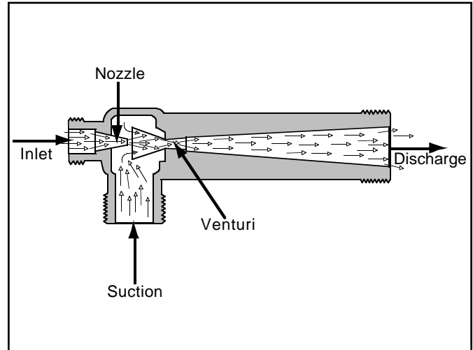
Figure 1—Typical ejector configuration for use in water ejector drafting operations.
