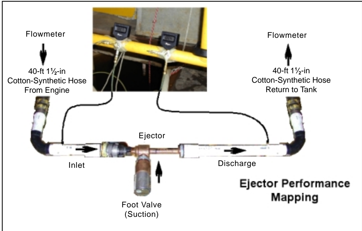
Figure B1—Equipment setup for mapping ejector performance.
