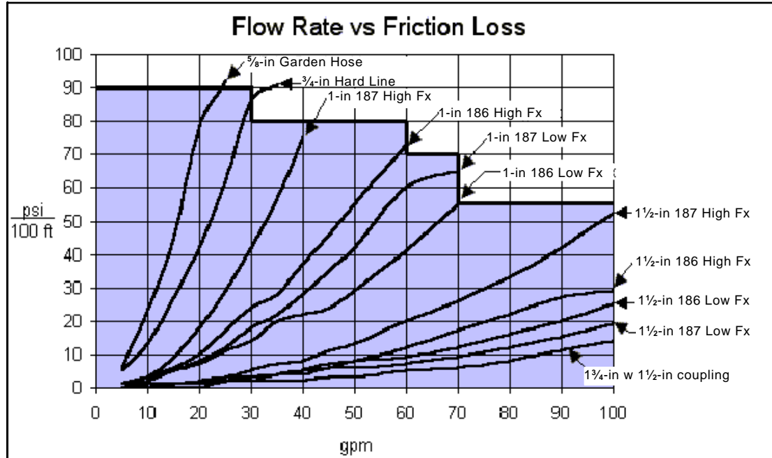
Figure D1—Flow rate versus friction loss per 100 ft of forestry hose and hose on the Forest Service 5100-186 and 5100-187 Qualified Products Lists for forestry hose.
