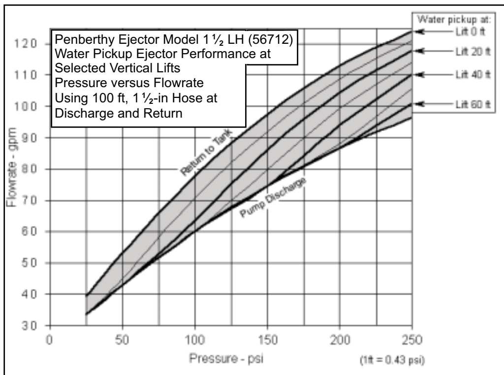
Figure A7—Penberthy Model 1½ LH (56712) water pickup ejector performance graph.
