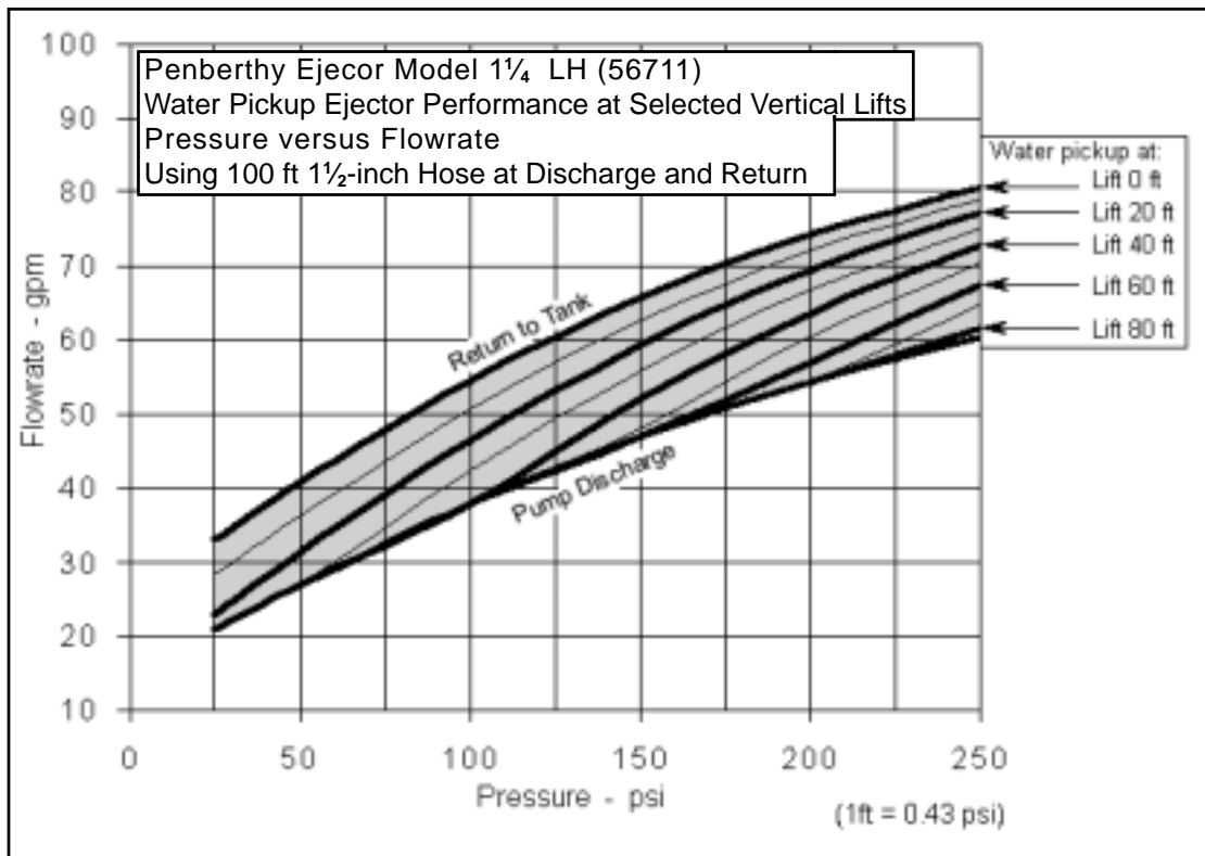
Figure A6—Penberthy Model 1¼ LH (56711) water pickup ejector performance graph.
