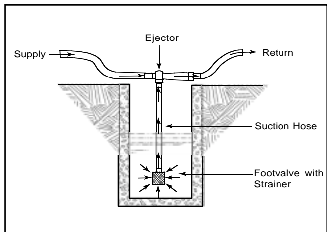
Figure 12—Ejectors can be used to draft water from a well.
