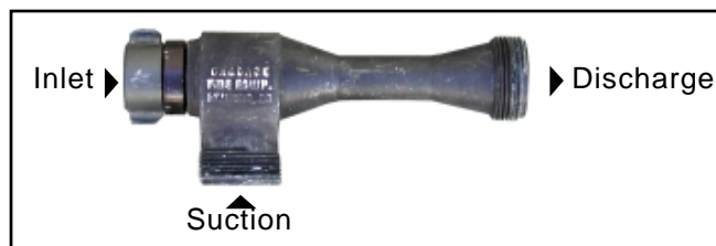
Figure E2—Cascade Ejector Model 14726 configuration.
