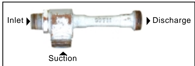
Figure E5—Penberthy Ejector Model 1¼ LM configuration.
