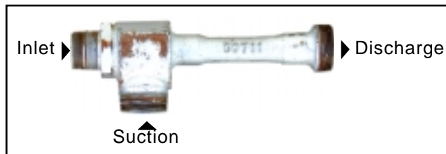
Figure E7—Penberthy Ejector Model 1½ LH configuration.
