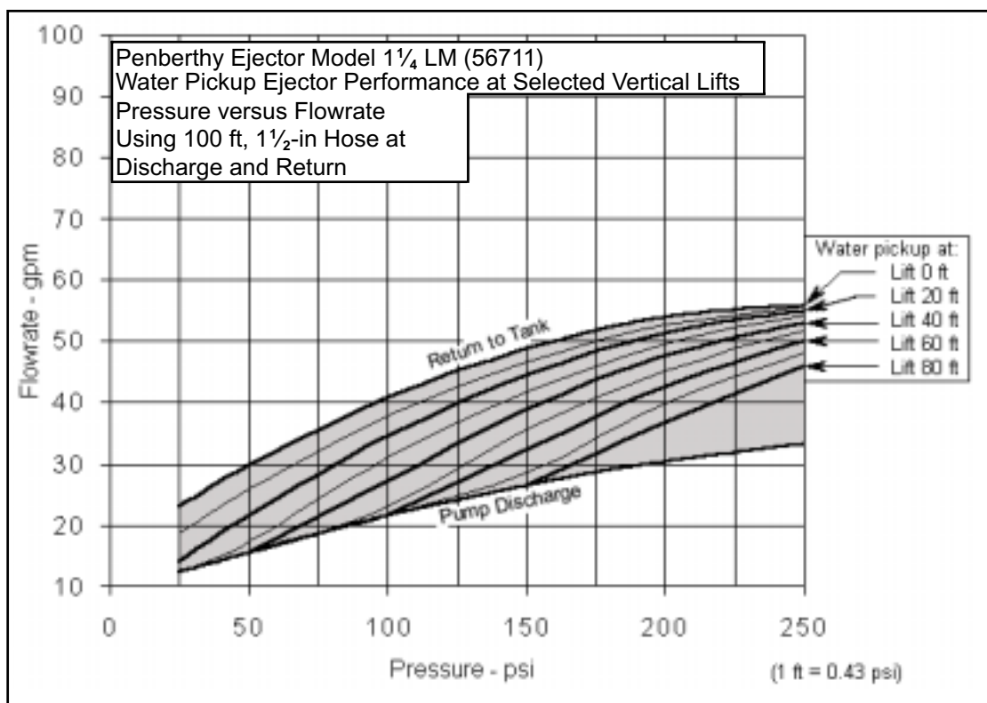
Figure A5—Penberthy Model 1¼ LM (56711) water pickup ejector performance graph.
