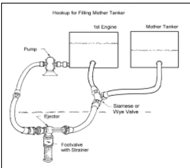
Figure 10—Ejector drafting operation for refilling the primary and mother tanks simultaneously.
