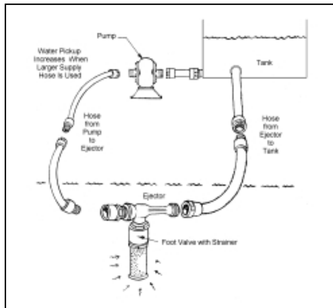
Figure 2—Ejector setup from the engine to water source and return.
