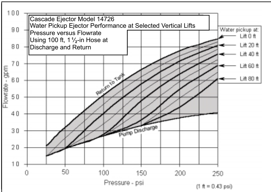
Figure A2—Cascade Model 14726 water pickup ejector performance graph.
