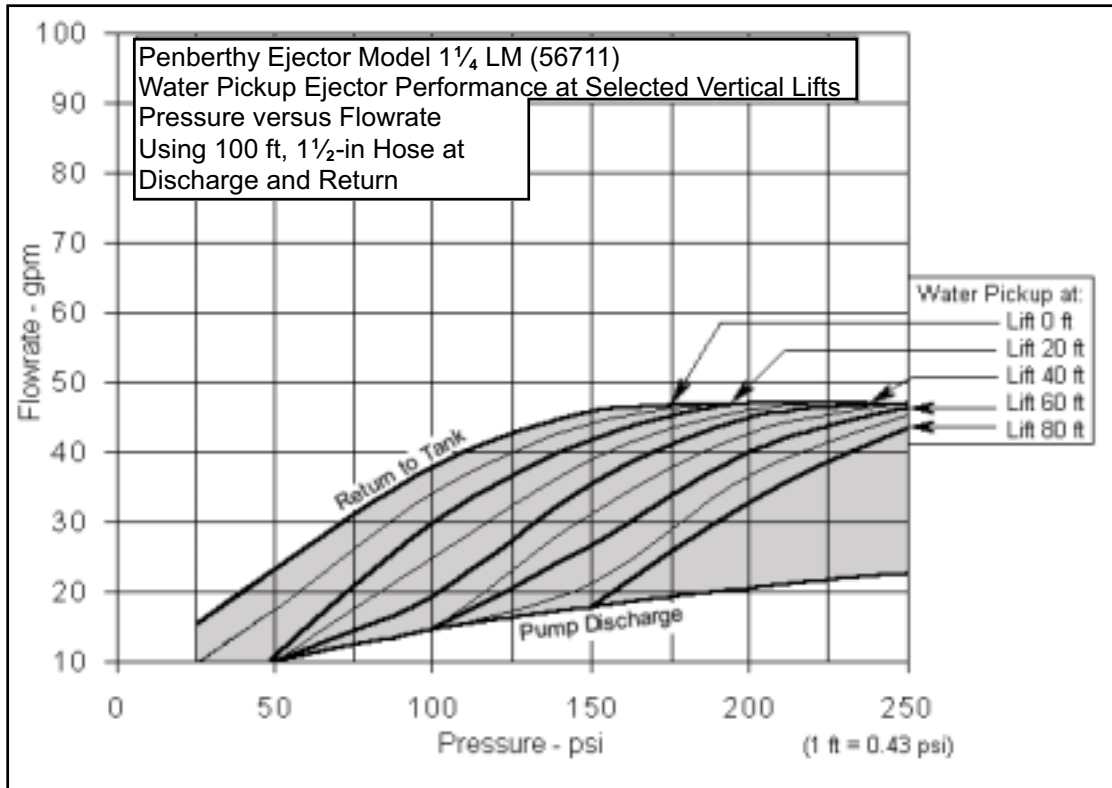
Figure A1—Penberthy Model 1¼ LL (56711) water pickup ejector performance graph.
