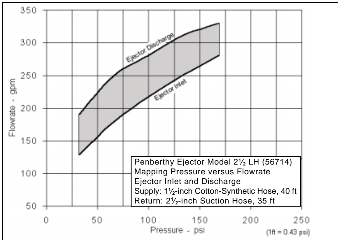
Figure A8—Penberthy Model 2½ LH (56714) mapping pressure versus flowrate graph.
