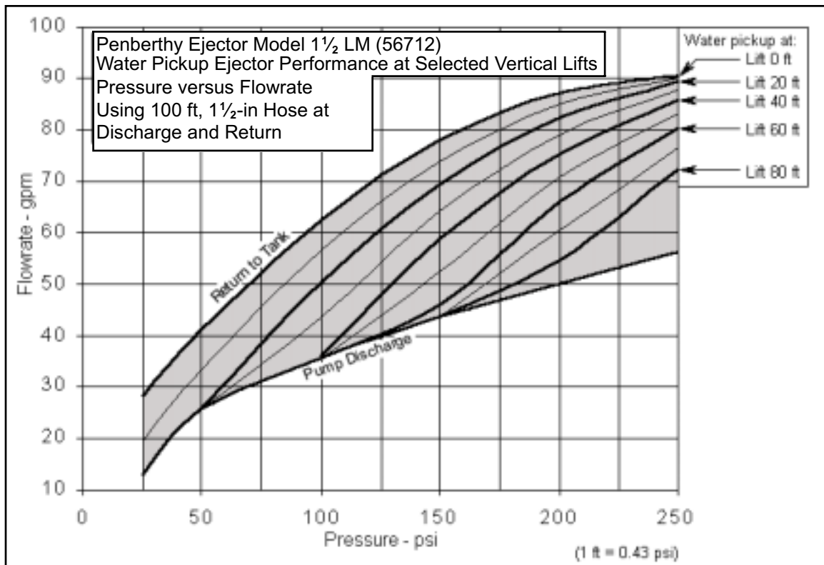
Figure A4—Penberthy Model 1½ LM (56712) water pickup ejector performance graph.
