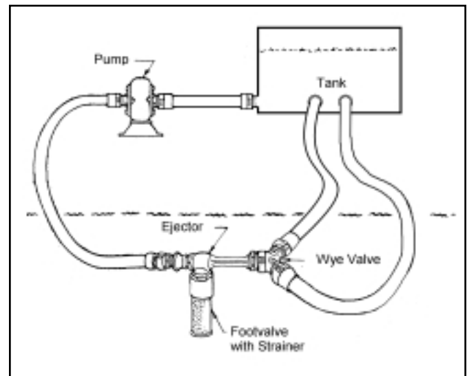
Figure 13—Friction loss is reduced by using dual return lines.
