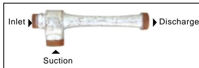
Figure E9—Penberthy Ejector Model 2½ LH configuration.
